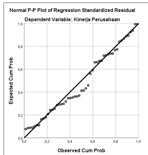
Gambar 4.1 Normal P-P of Regression Standardized Residual
