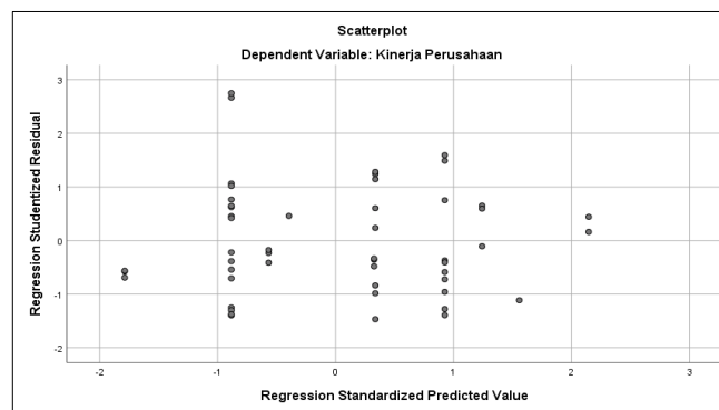
Gambar 4.2 Scatterplot
