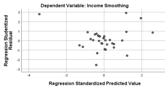
Scatterplot
