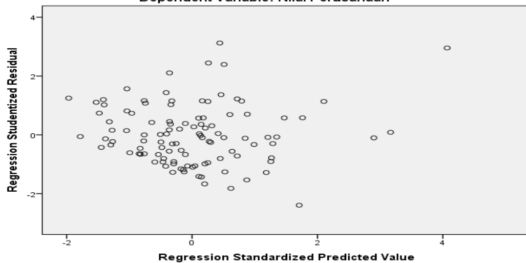
Scatterplot
